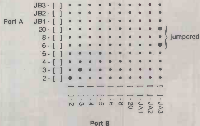
Figure 1. Folding back a voltage on line 20 to line 6 using jumper area 3.
